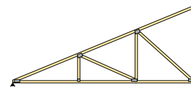
Mono truss
